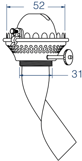
Burner 1''' Type: Flat wick Wick: 25 x 230
