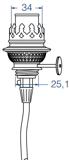
Imitation Burner 6''' Lamp-holder E14
