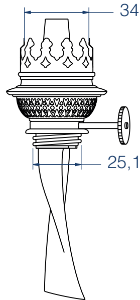
Burner 6''' Type: Round Wick: 35 x 230
