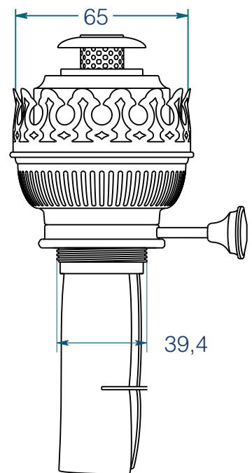
Burner 20''' Type: Ideal burner Wick: 90 x 230
