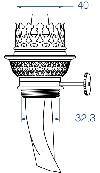
Burner 10''' Type: Round Wick: 48 x 230
