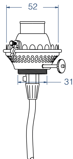
Imitation Burner 1''' Lamp-holder E14
